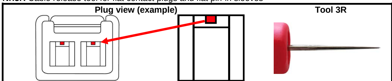
Nr.3R Cable release tool for flat contact plugs and flat pin-in sleeves
