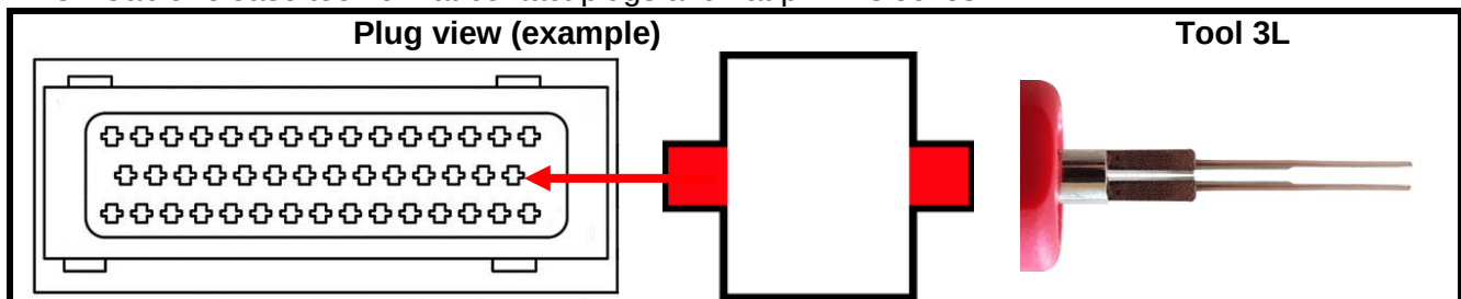
Nr.3L Cable release tool for flat contact plugs and flat pin-in sleeves
